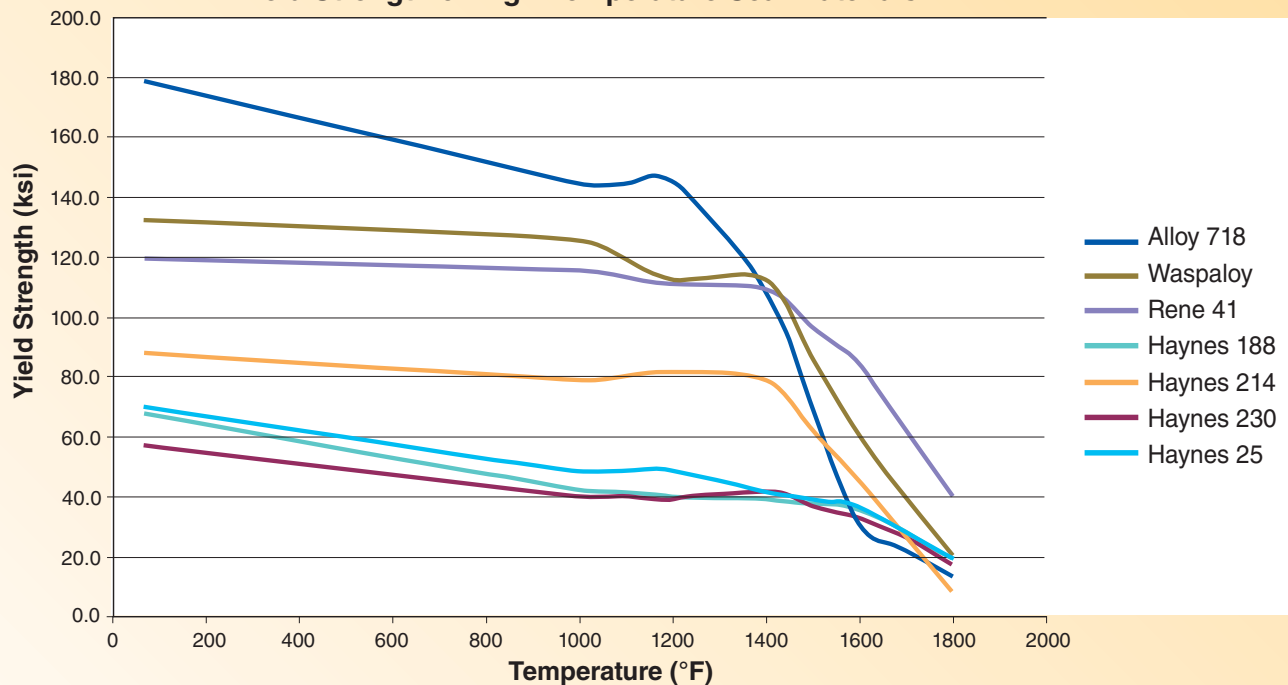
Yield Strength of High-Temperature Seal Materials
